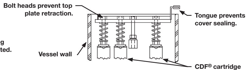
Position 1 - Before Tightening
