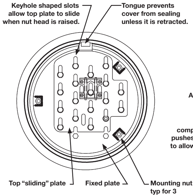
Plan View - Interlock Assembly
